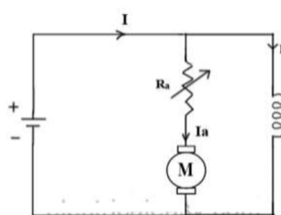
Armature Control Method
