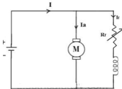
Flux Control Method
