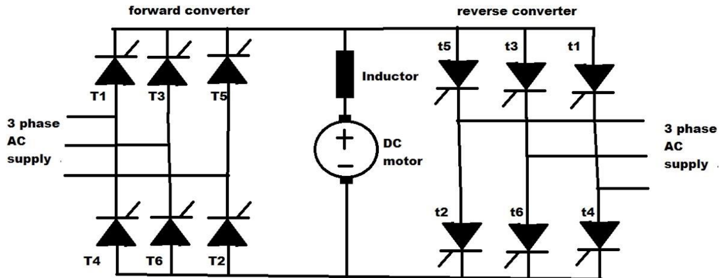
Dual converter for four quadrant operation of dc motor
