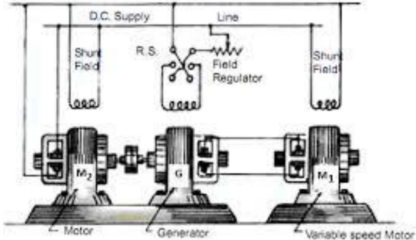
WARD LEONARD SYSTEM OF SPEED CONTROL
