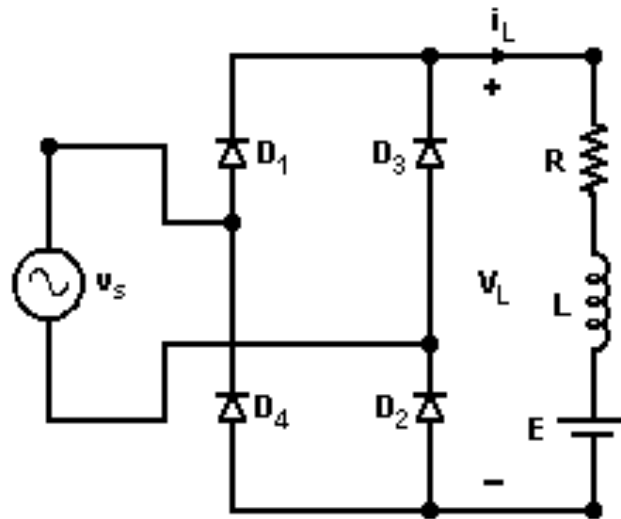
(a) Circuit
