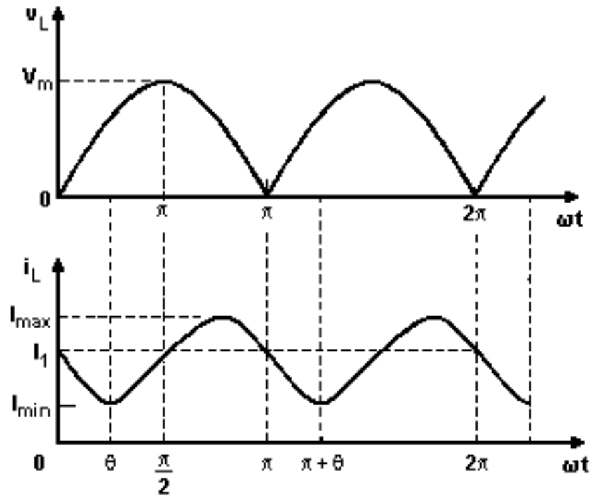
(b) Waveforms
