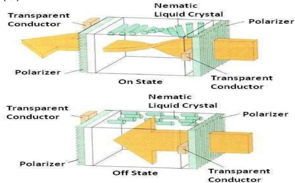
Fig. 1.10: - Light twisting shutter effect used in design of most LCD.
