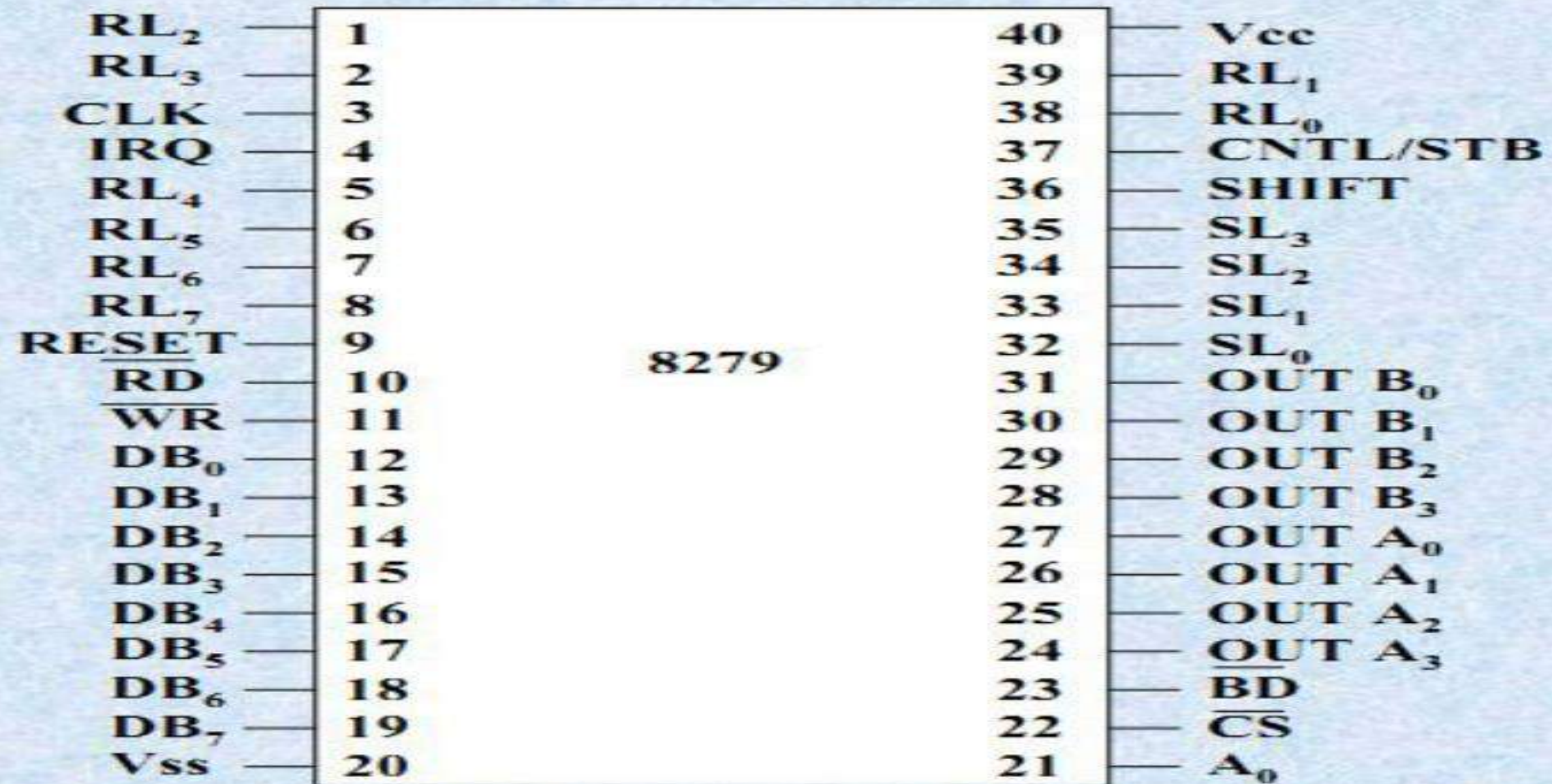
8279 Pin Configuration
