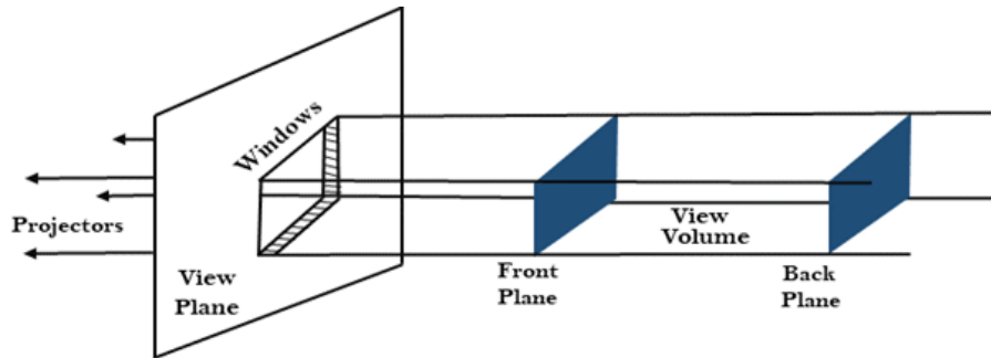
(a) Viewing Volume in orthographic projection
