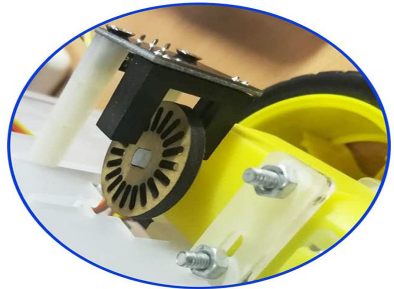
Encoder + Wheel Fixture For DC Motor Shaft
