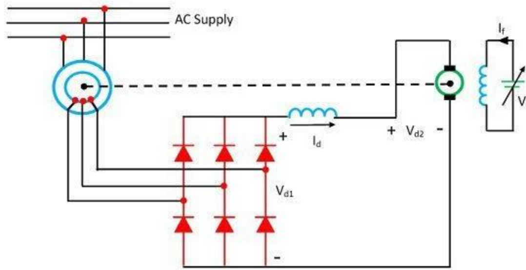
Static Kramer Drive Circuit
