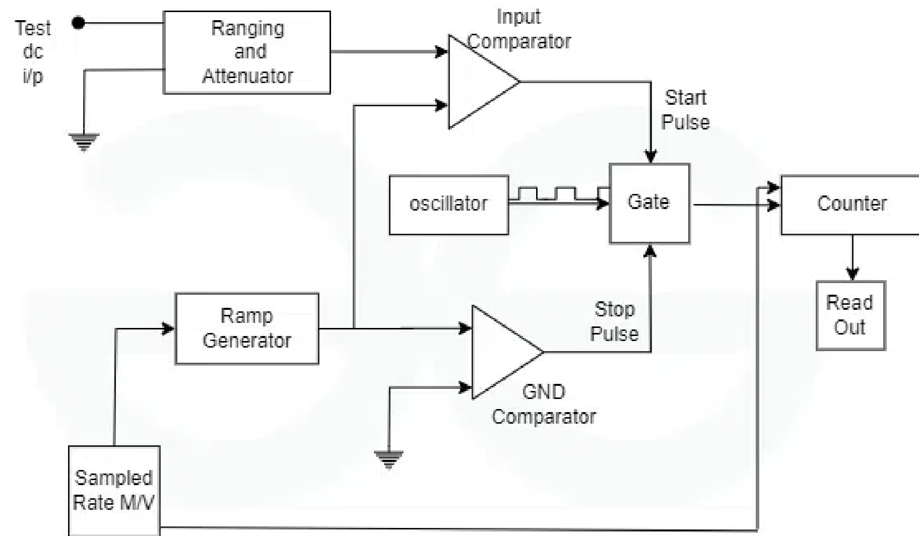
Working Principle of Digital Voltmeter
