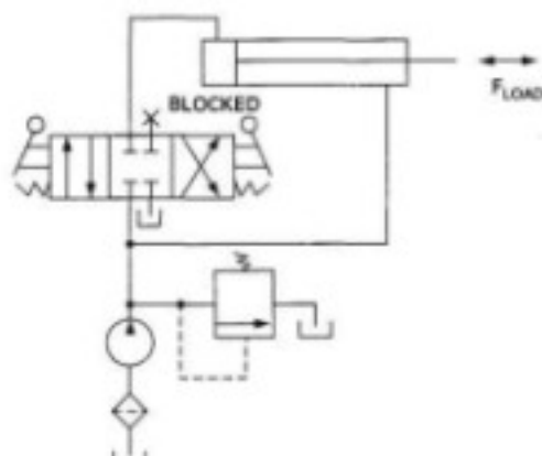
Complete circuit.
