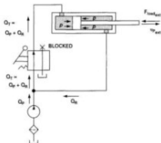
Partial circuit showing flow paths during cylinder extension stroke.
