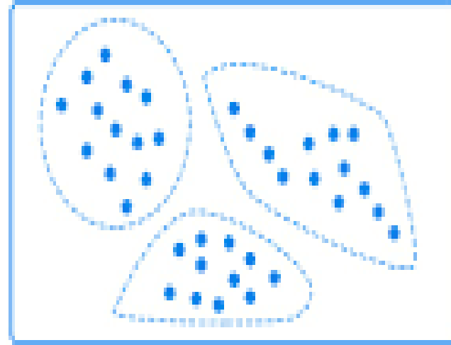
Unsupervised learning
