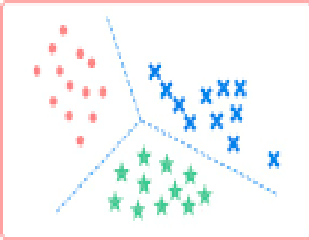
Supervised learning
