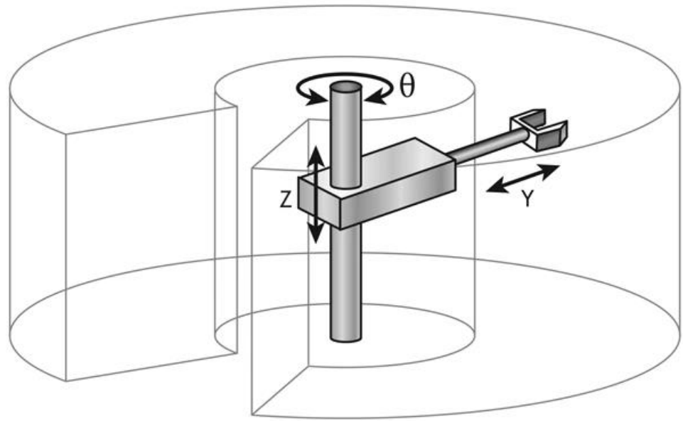
Cylindrical robot
