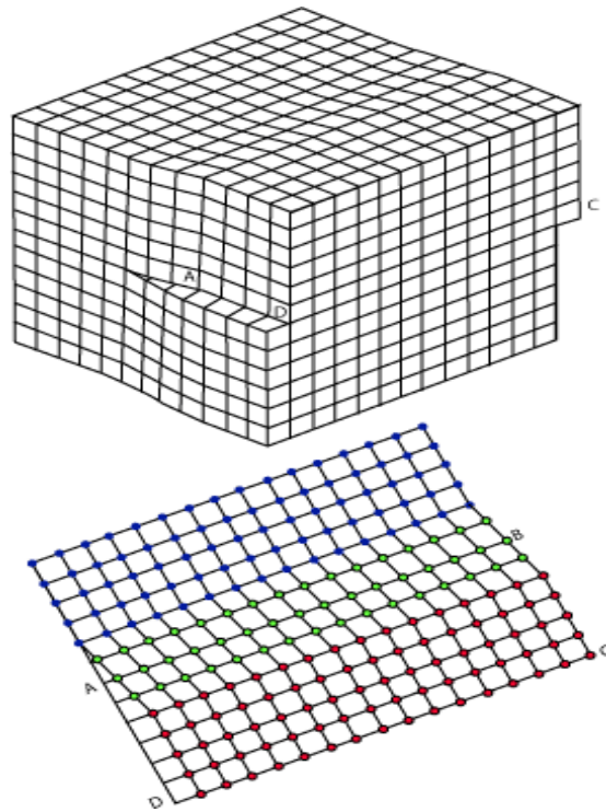
Fig 7. Screw dislocation
