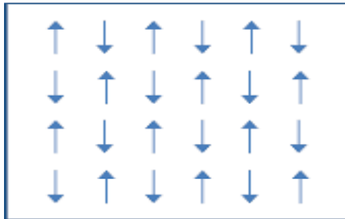
Antiferromagnetic ordering
