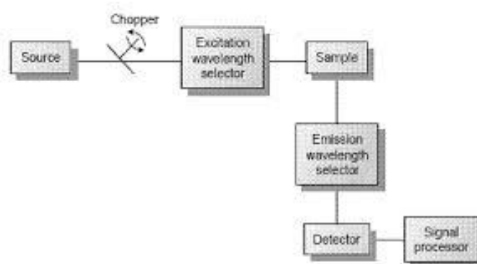
Block diagram of Atomic absorption spectrophotometer.
