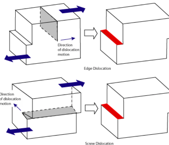
Fig 8: to show edge and screw dislocations
